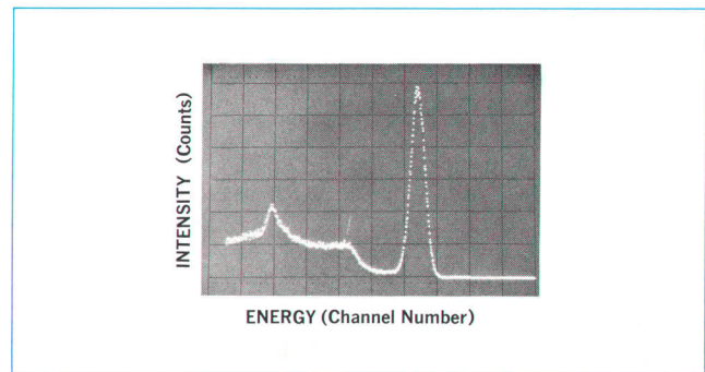
Fig. 1. Gamma-ray spectrum of Cs^{137} as seen by a scintillation detector is typical of multichannel-analyzer results. The information of interest—the energy and intensity of each peak—can't be read directly; it has to be extracted by computation.
